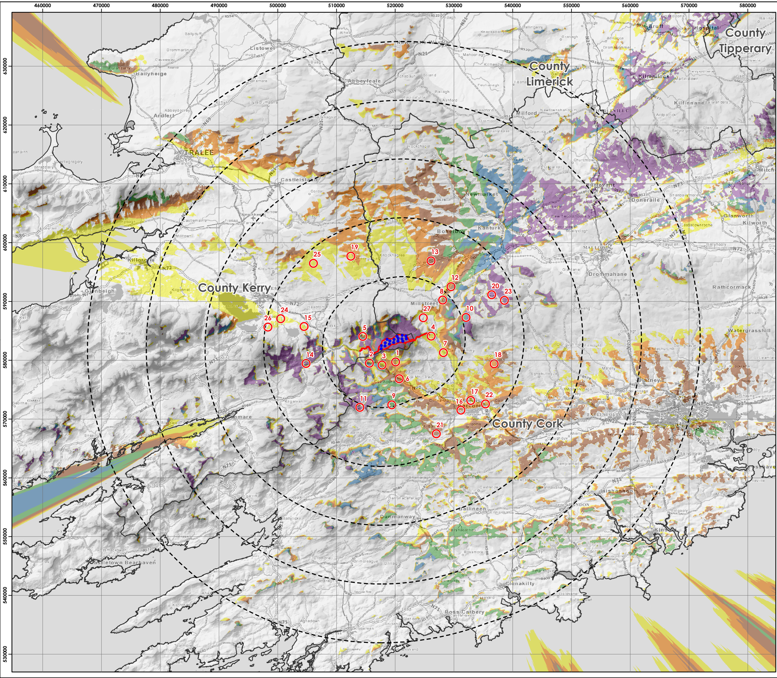
Figure 6-2a Zone Of Theoretical Visibility 200m Blade Tip Height to 50km
